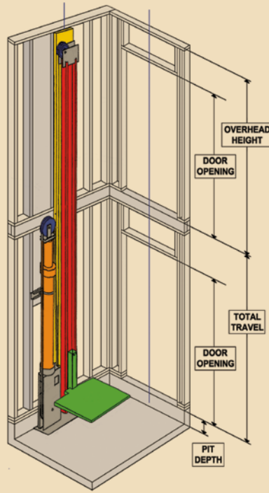
Hydraulic
